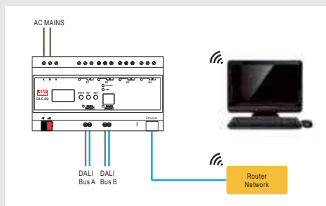
Commissioning the DLC-02 via web browser
