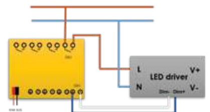
3. DC 1-10V Driver
