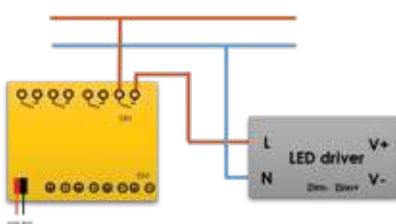
1. Non-dimmable Driver
